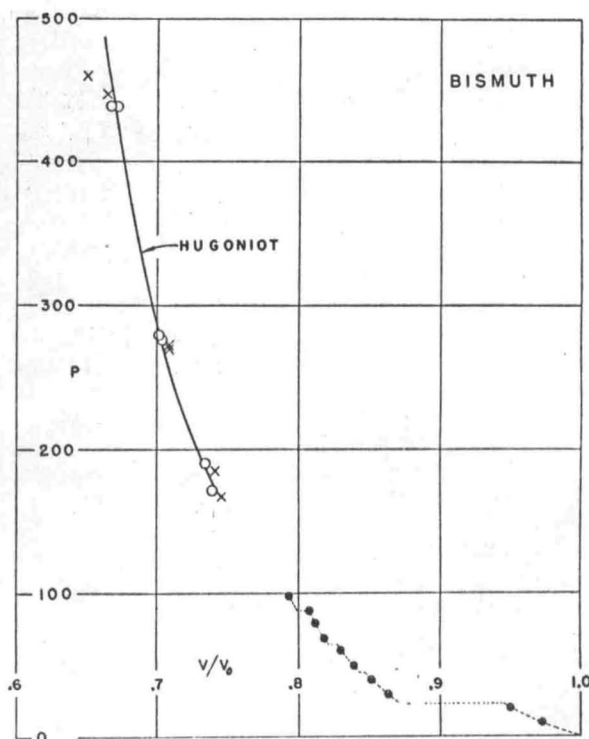
FIG. 4. Pressure-compression curves for bismuth. See caption to Fig. 3.
