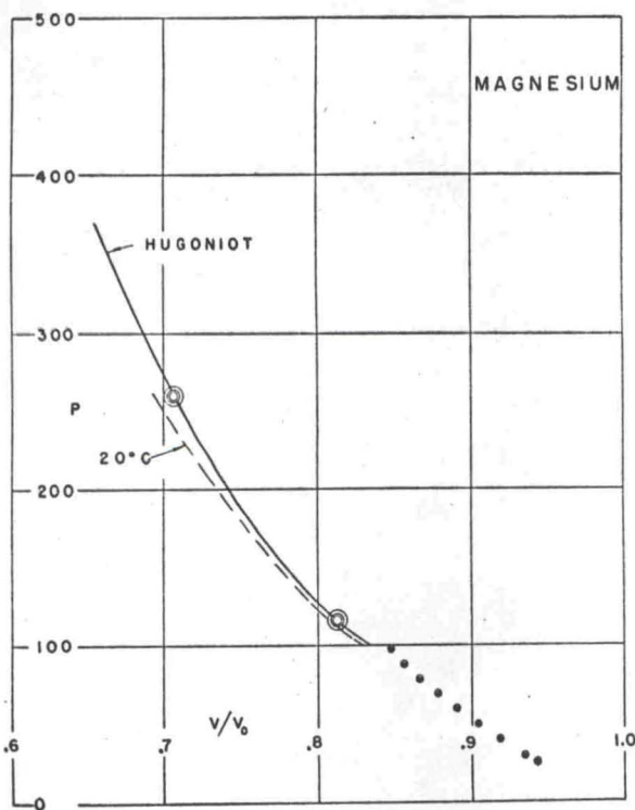
FIG. 12. Pressure-compression curves for magnesium. See caption to Fig. 3.
