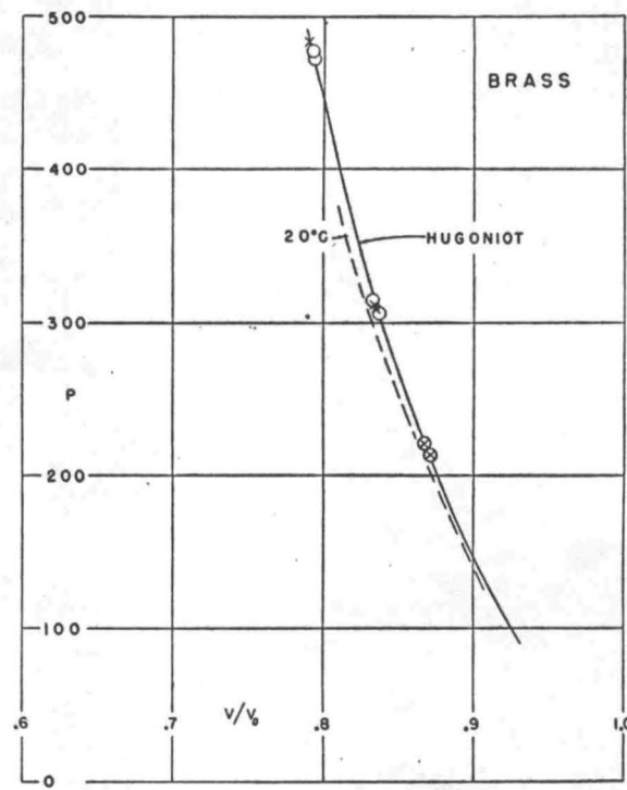
FIG. 21. Pressure-compression curves for brass. See caption to Fig. 3.
