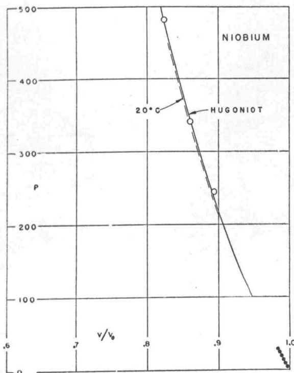
FIG. 23. Pressure-compression curves for niobium. See caption to Fig. 3.
